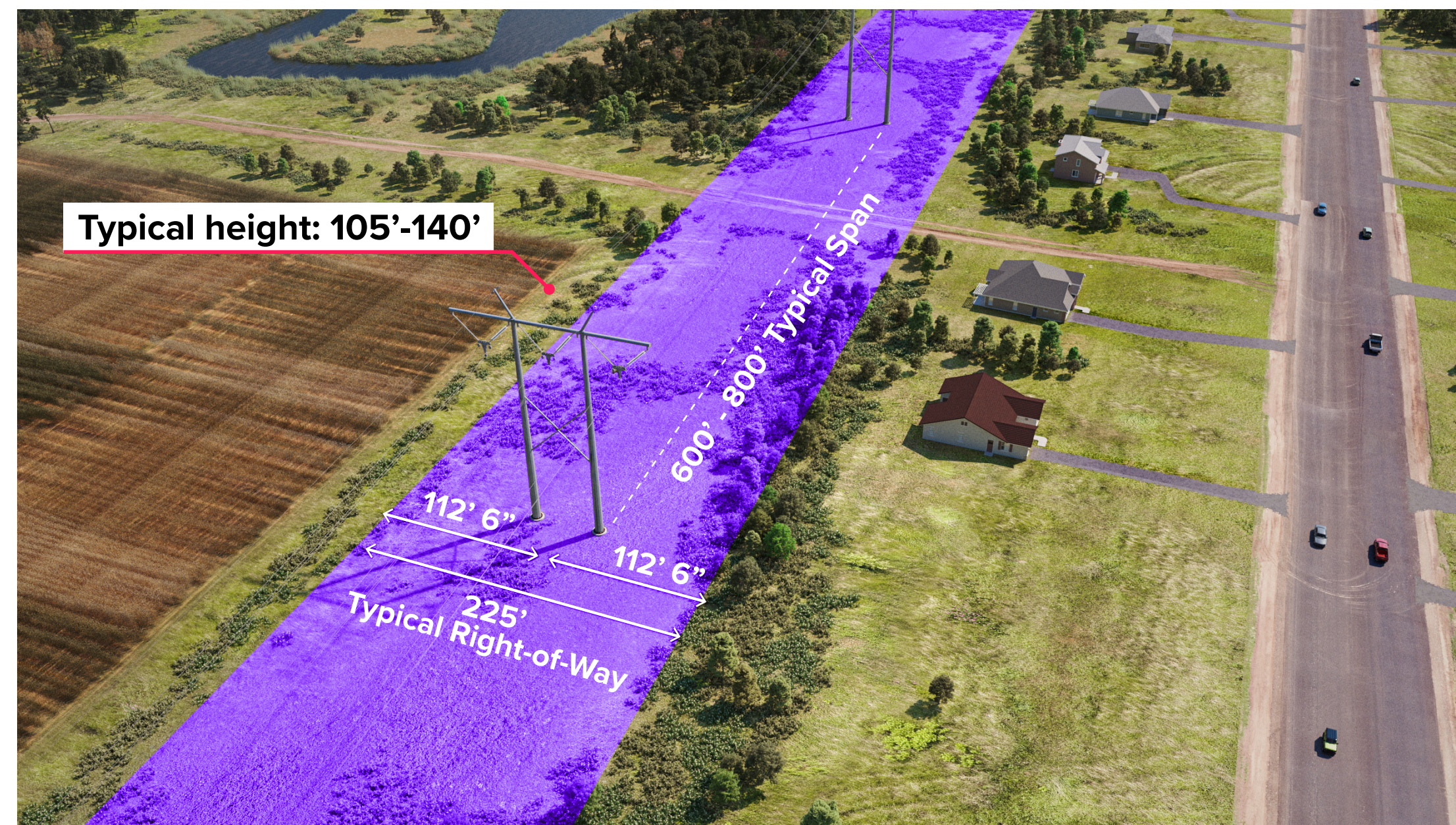
Structure installation
